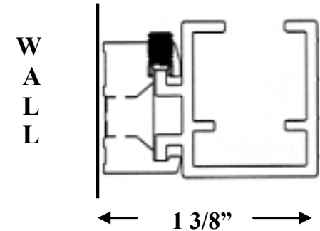
STANDARD TRACK SC2000
